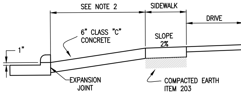
SECTION A-A STANDARD COMBINED CURB AND GUTTER SECTION
