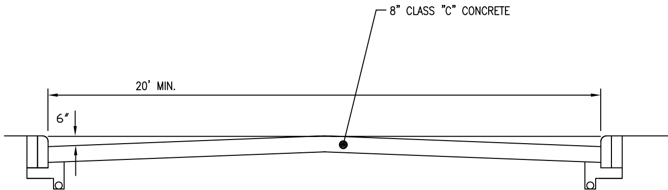
SECTION A-A THROUGH CROWNED PAVEMENT
