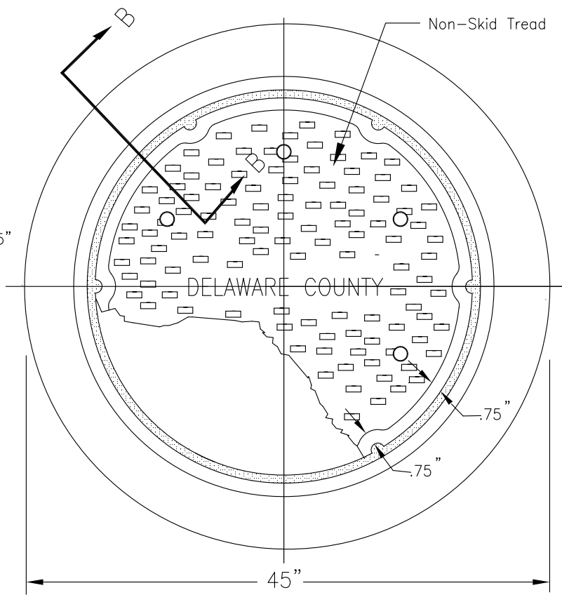
TOP VIEW OF ASSEMBLY
