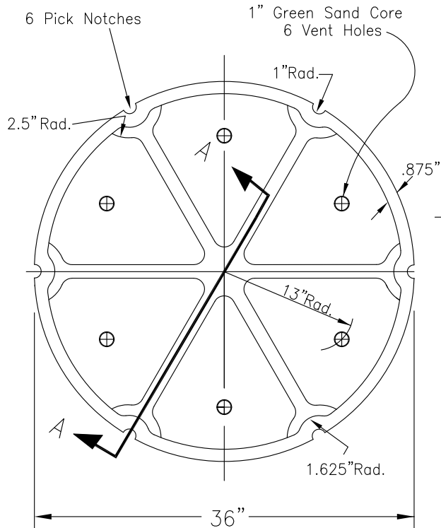
BOTTOM VIEW OF COVER (SEE SHEET 2 OF 2 FOR ALTERNATE DESIGN)
