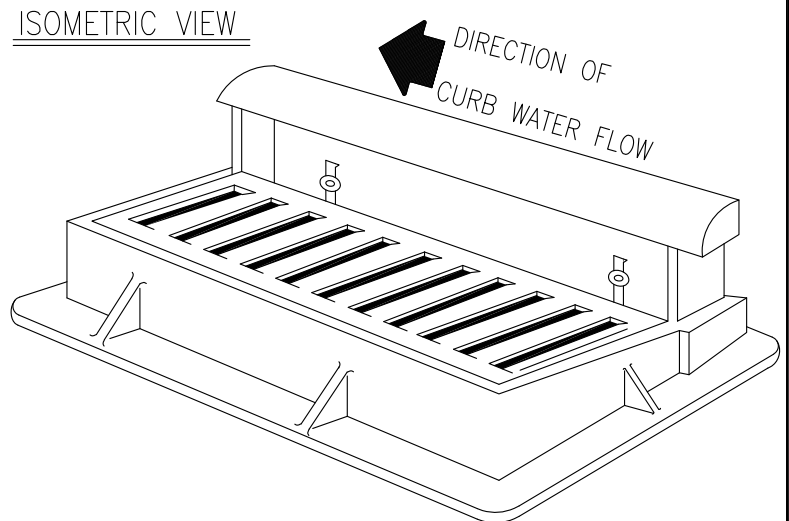
FRAME, CURB BOX and GRATE ASSEMBLY APPROX. WEIGHT = 525 lbs.
