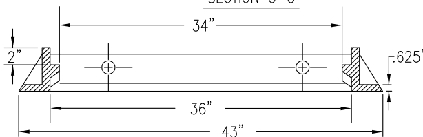
FRAME, CURB BOX and GRATE ASSEMBLY APPROX. WEIGHT = 525 lbs.
