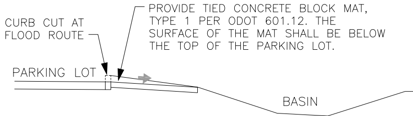
FLOOD ROUTES DOWNSTREAM OF PARKING LOTS
