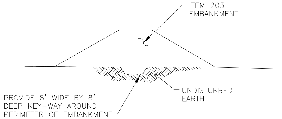
EMBANKMENT KEYWAY DETAIL
