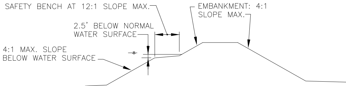
SAFETY BENCH DETAIL
