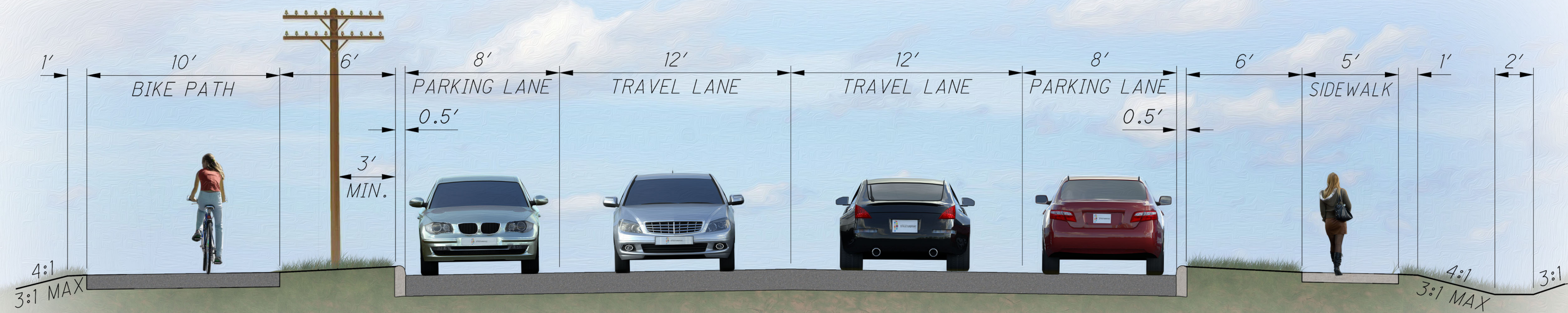
ALTERNATIVE 3A - WITH ON-STREET PARKING
