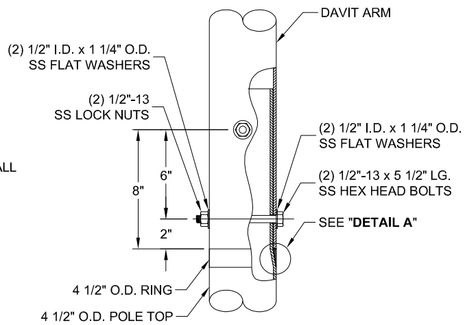
CONNECTION DETAIL
