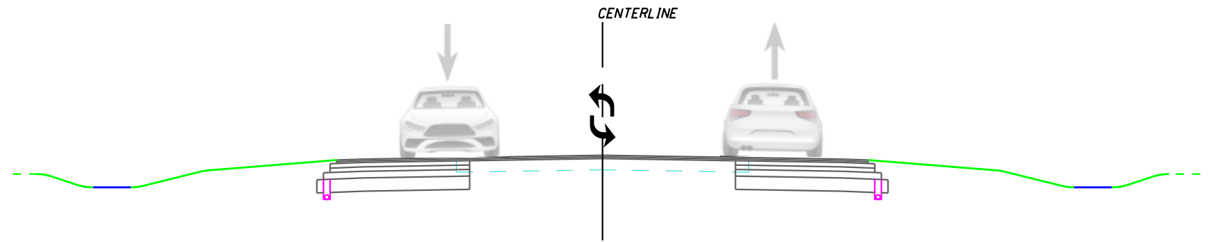
NORMAL SECTION - UNCURBED WIDENING
