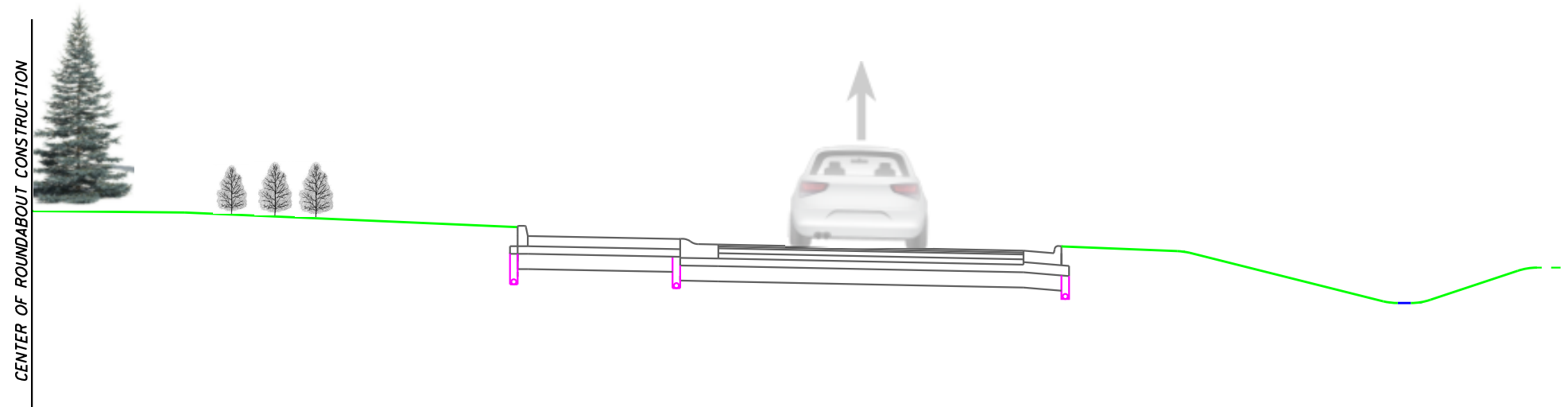
ROUNDABOUT SECTION
