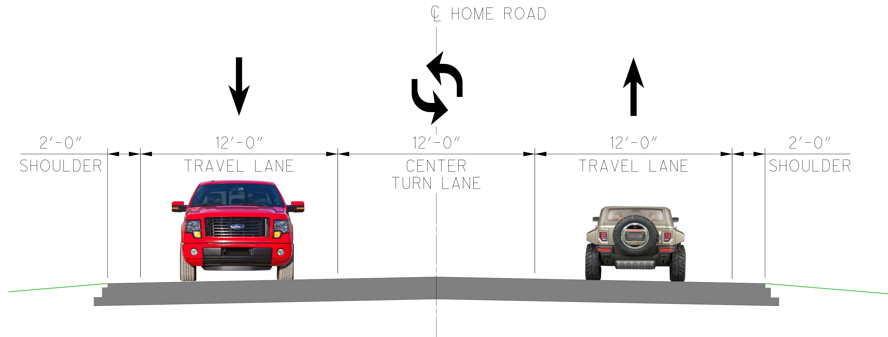
3-LANE SECTION
