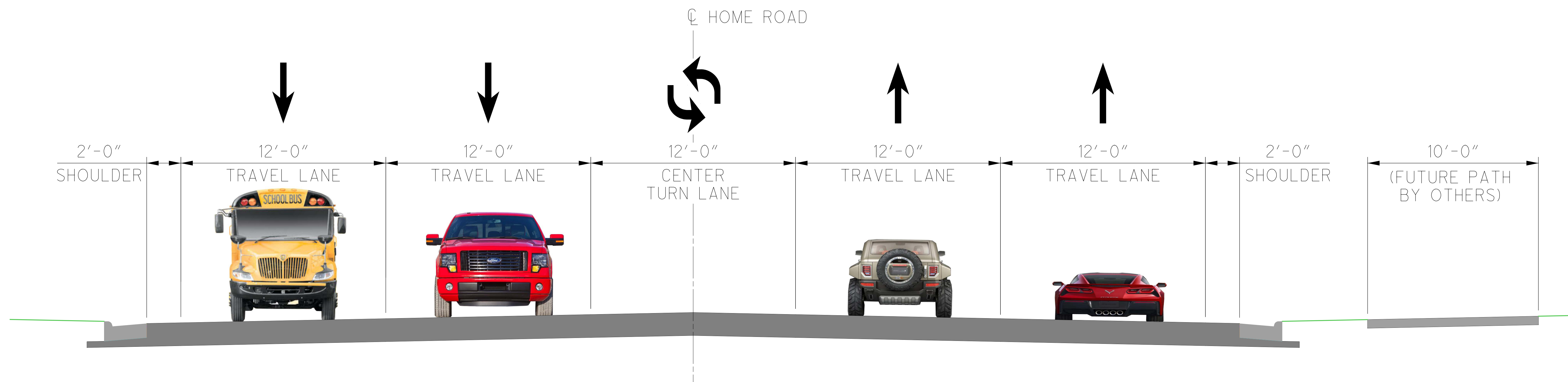
5-LANE SECTION
