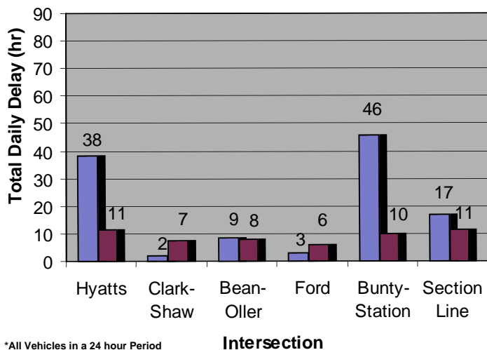
2009 Daily Intersection Delay*
