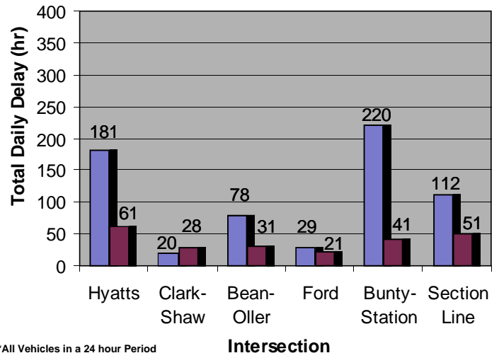
2030 Daily Intersection Delay*
